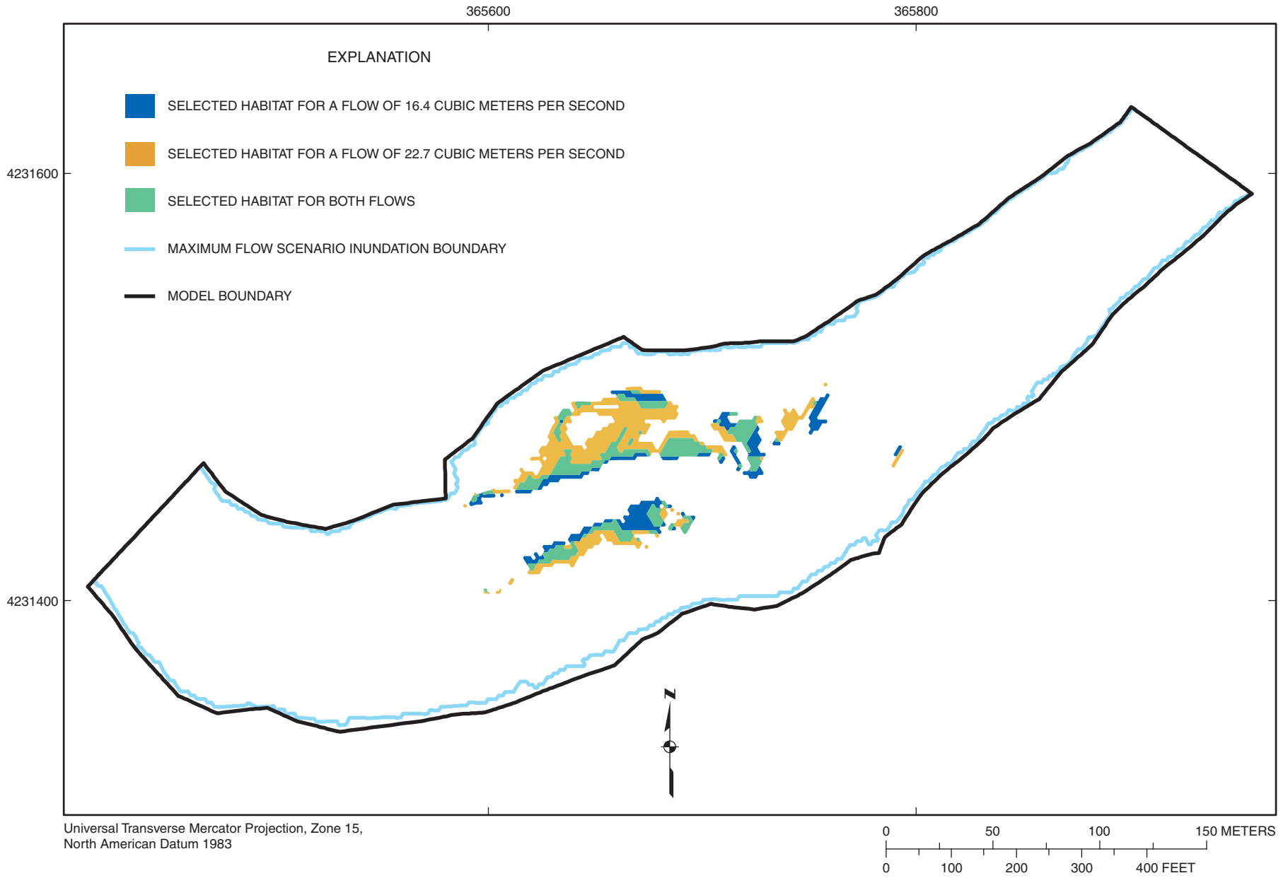
Figure 4-82. Selected habitat area distribution for habitat category 20 (flathead catfish) at flows of 16.4 and 22.7 cubic meters per second at Marais des Cygnes River site MDC2.
